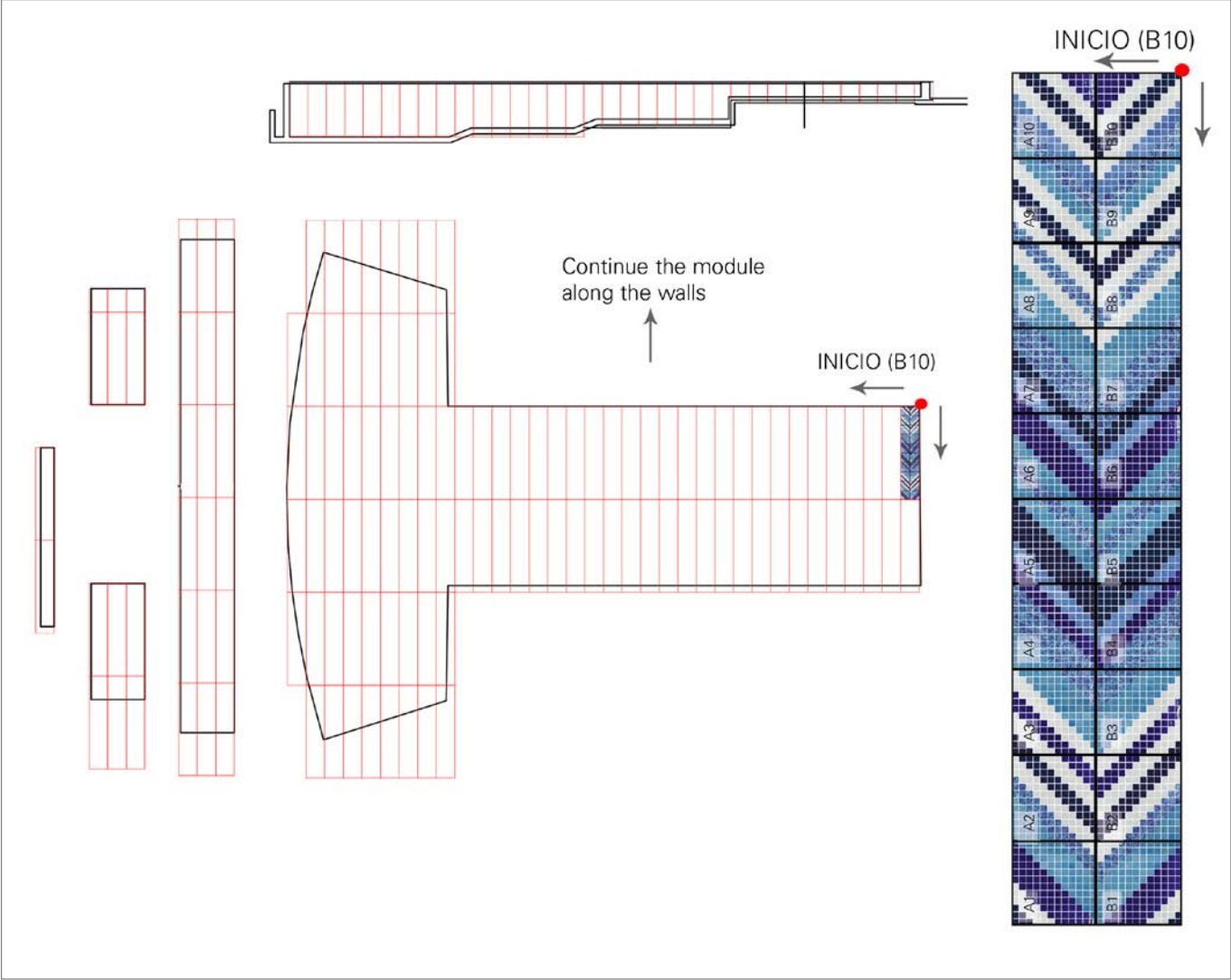
Installation Drawing
